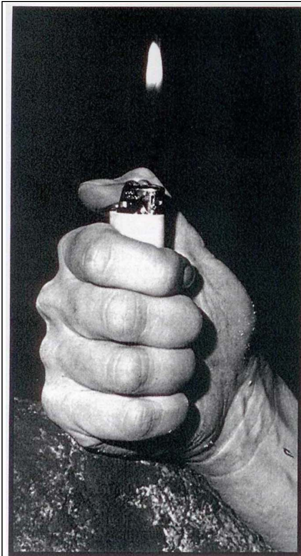
The flame test being performed by Jenny Whitby in Grill Cave at Bungonia NSW, Australia. The CO_2 on this occasion was measured at 5% with a Drager meter. Time to get out of the cave. Photo © Garry K Smith
